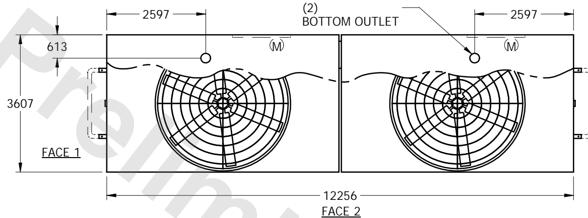
PLAN VIEW
