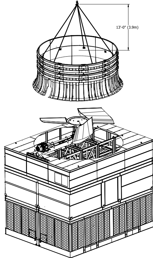
Figure 27 — Super Low Sound Fan Cylinder Rigging
