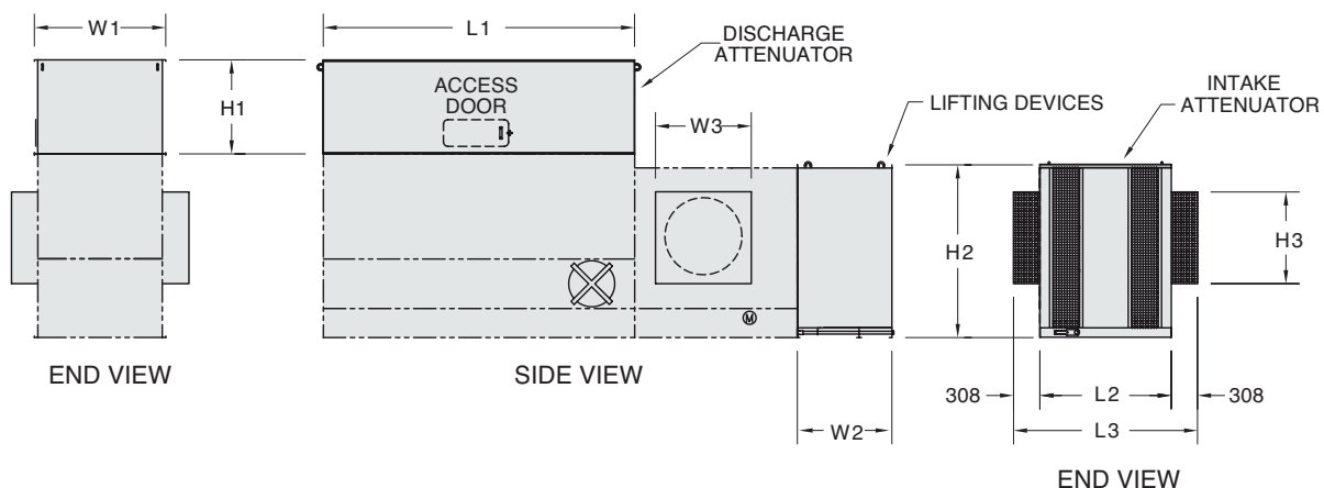
LRC Attenuation
