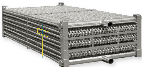
Thermal-Pak® Coil by EVAPCO
