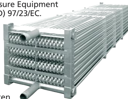
Thermal-Pak® Coil
