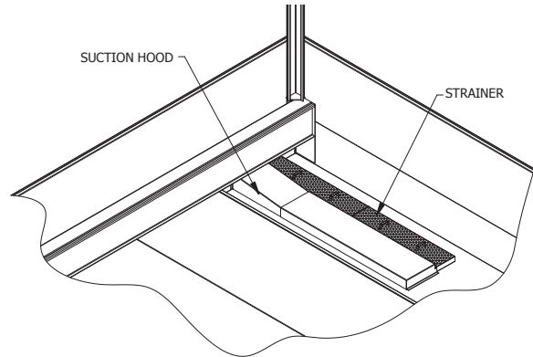
Figure 24 – Strainer Location
