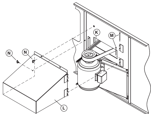
Figure 15 – External Motor Installation
