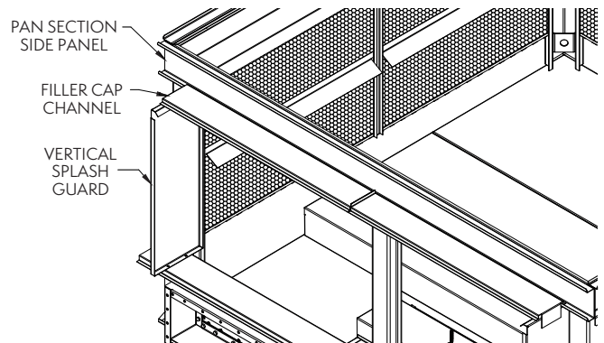
Figure 10 — Filler Cap Channel Assembly
