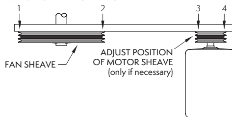
Figure 40 – Sheave Alignment Check
