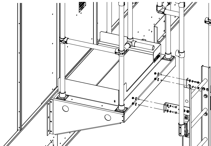
Figure 31 – Ladder Attachment Detail
