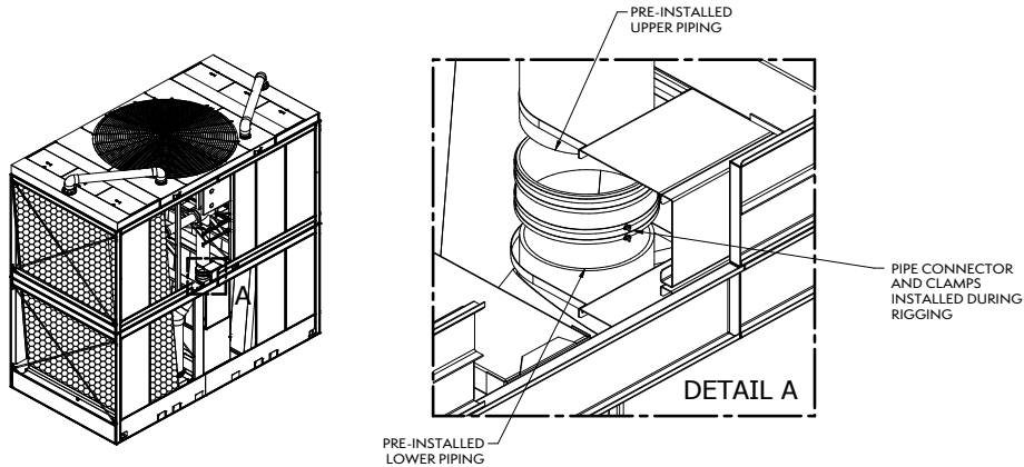
Figure 19 – Single Side Inlet
