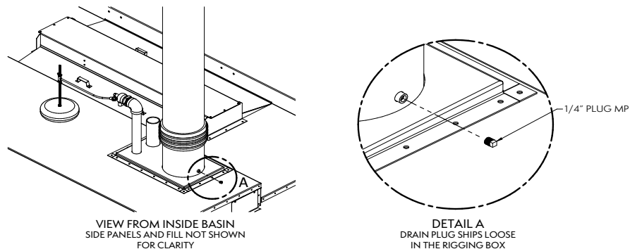
Figure 20 – Weep Hole
