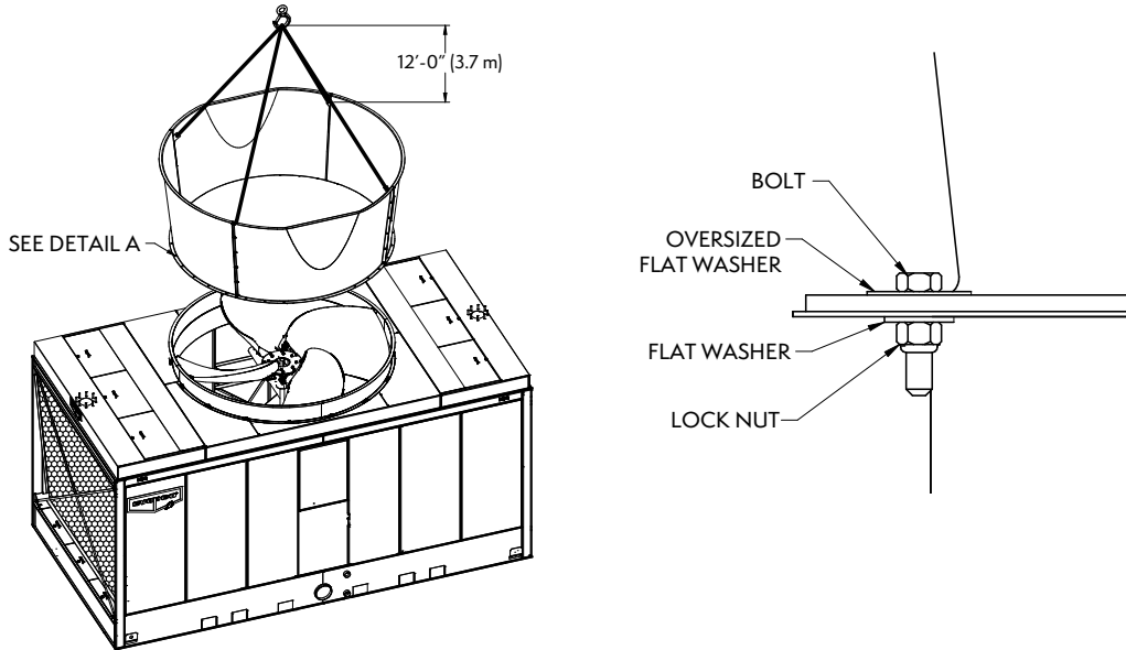
Figure 39 – VR Stack Rigging with a Super Low Sound Fan
