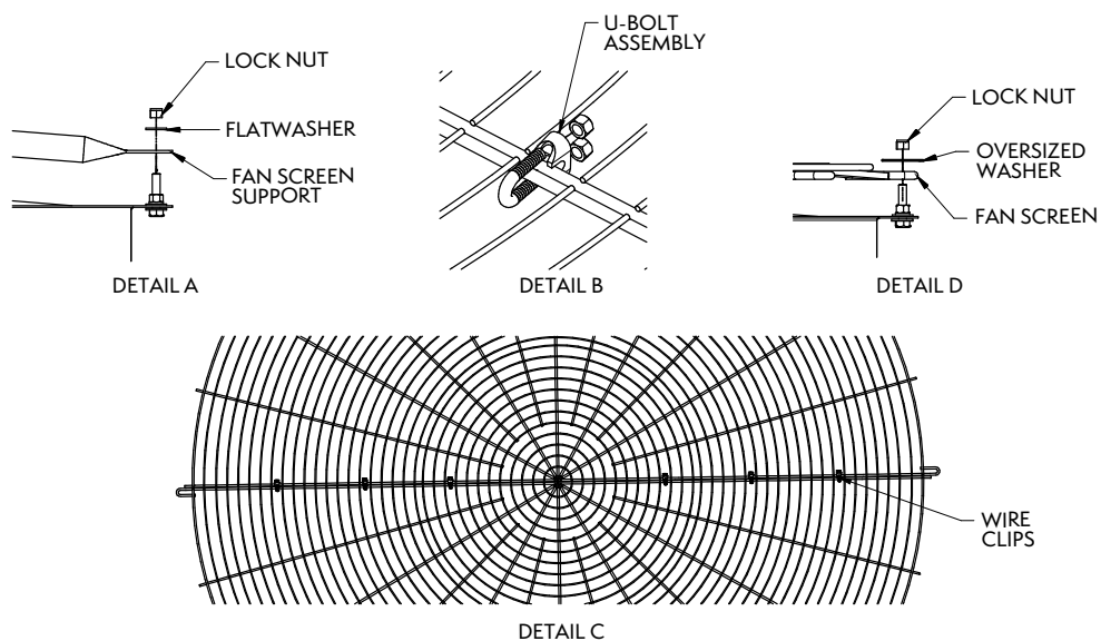
Figure 12 – Fan Screen and Fan Screen Support Frame
