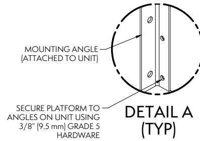
Figure 29 – Platform Securing Detail
