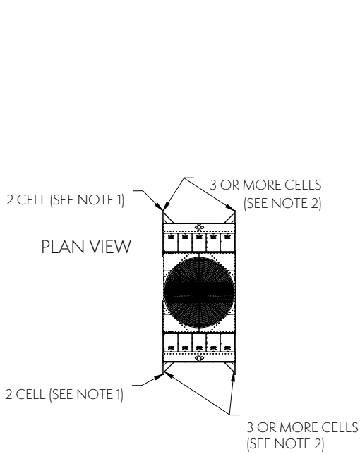
Figure 32 – Plan View of Firewall Installation
