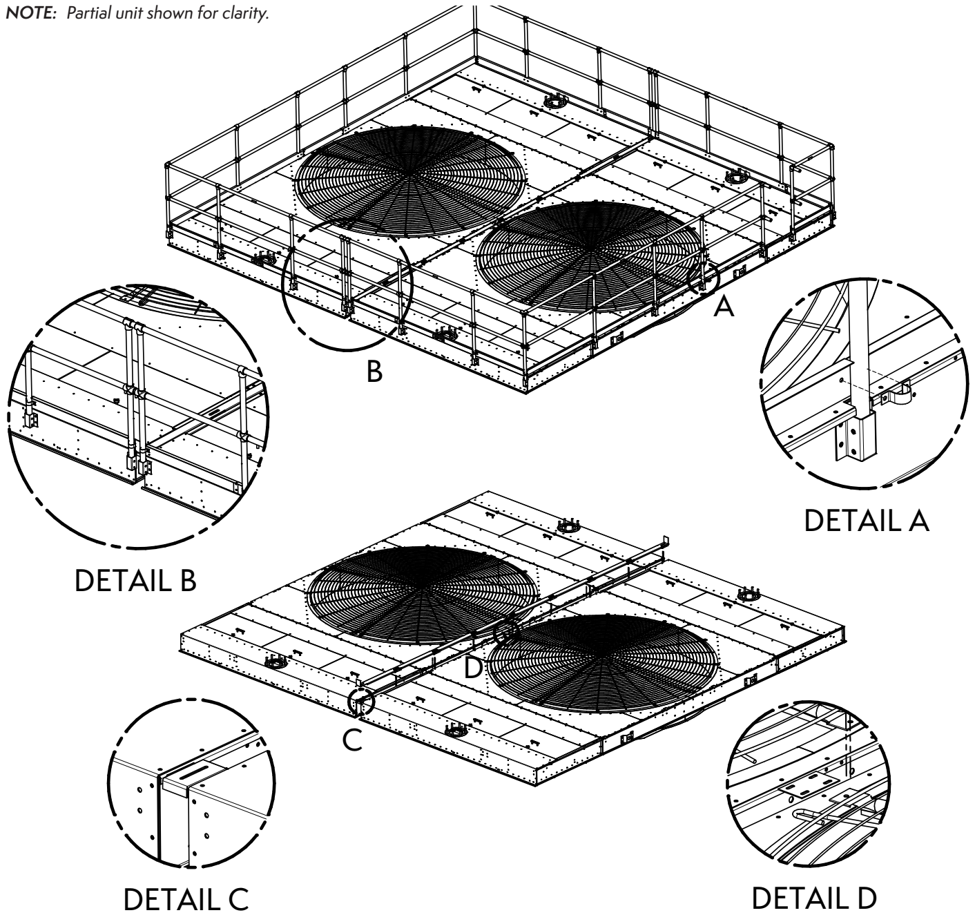
Figure 26 – Multi-Cell Top Channel Installations
