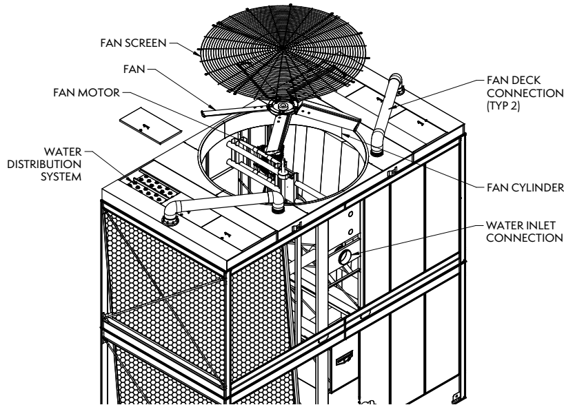
Figure 22 – Single Side Inlet
