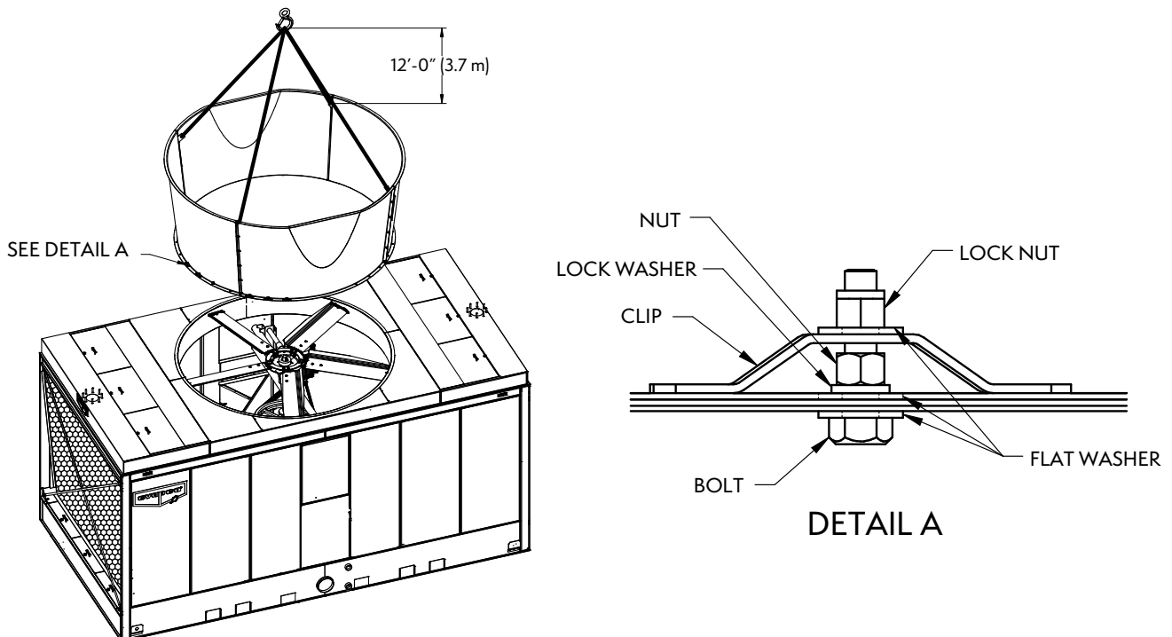
Figure 38 – VR Stack Rigging with a Standard Fan
