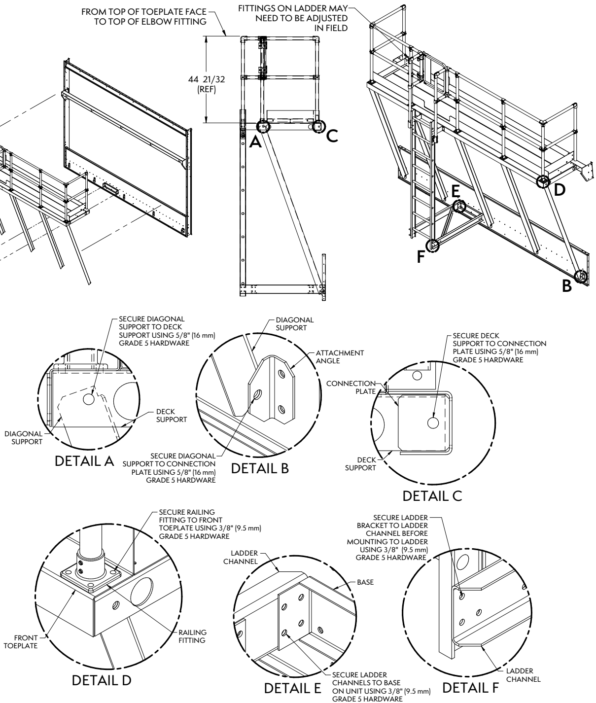
Figure 35 – Single Stack Louver Face Platform and Vertical Ladder Installation
