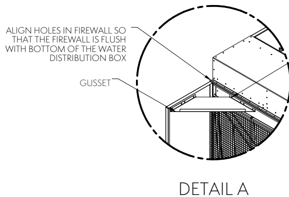
Figure 34 –DETAIL A of Firewall Installation
