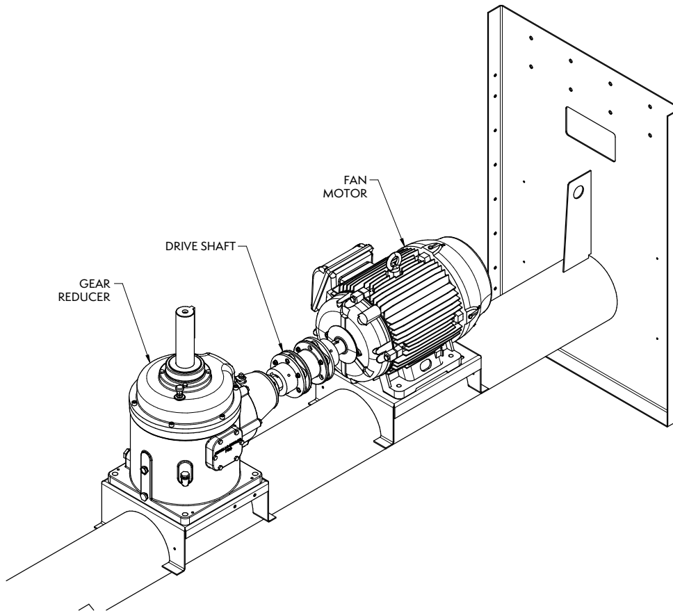
Figure 43 – Internal Motor Mount with Gear Drive and Super Low Sound Fan
