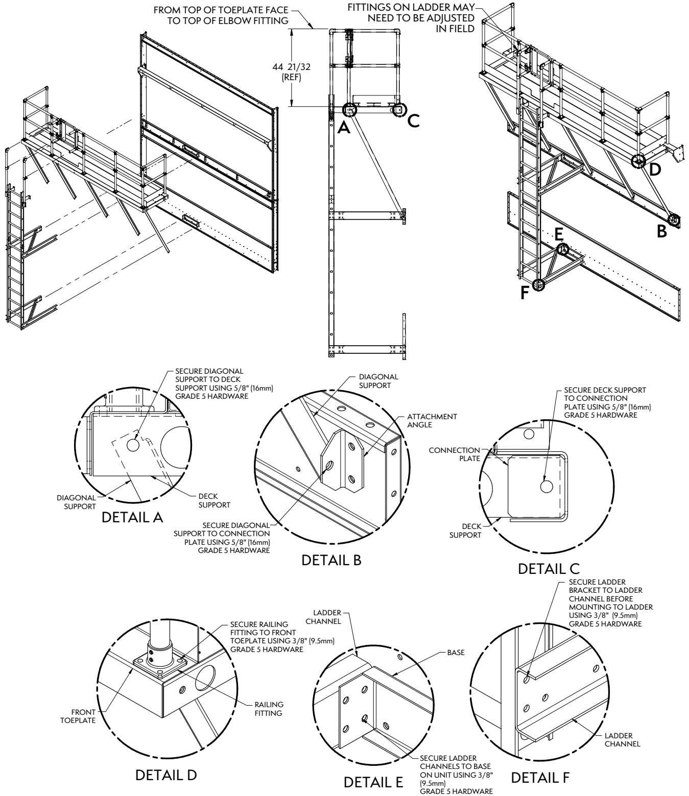
Figure 36 – Double Stack Louver Face Platform and Vertical Ladder Installation
