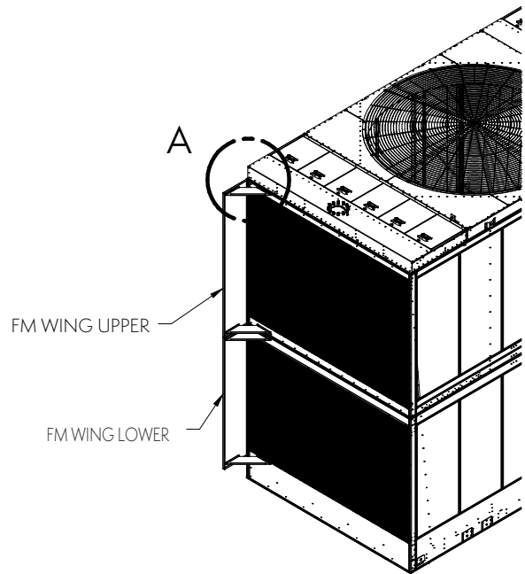
Figure 33 – Firewall Wing Arrangement
