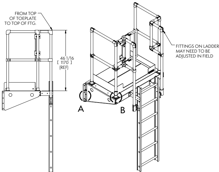
Figure 27 and 28 – General Basin Level Platform Arrangement
