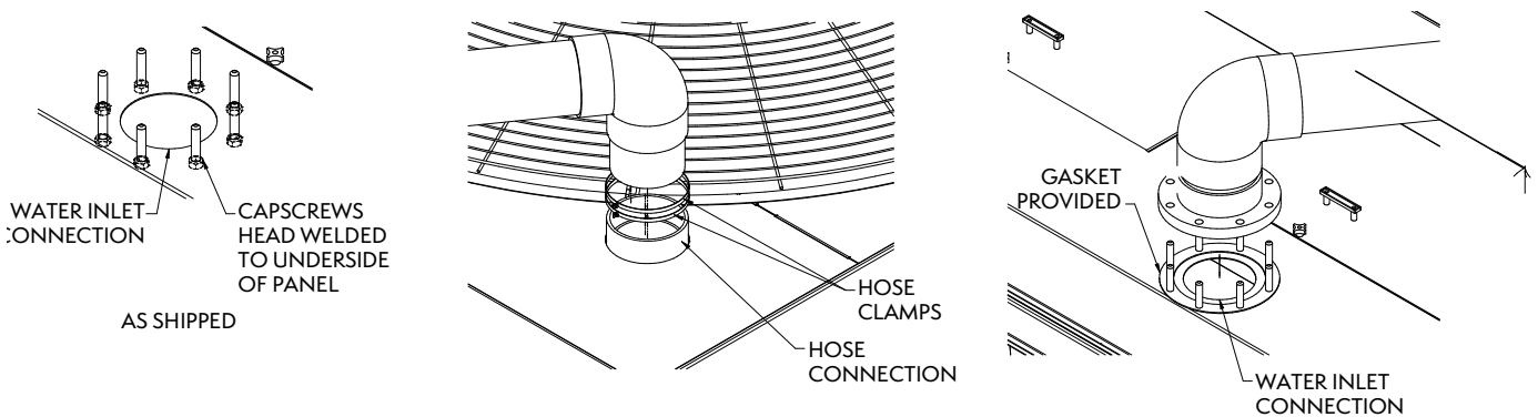
Figure 21 – ASME 150 Bolt Flange Pattern Setup
