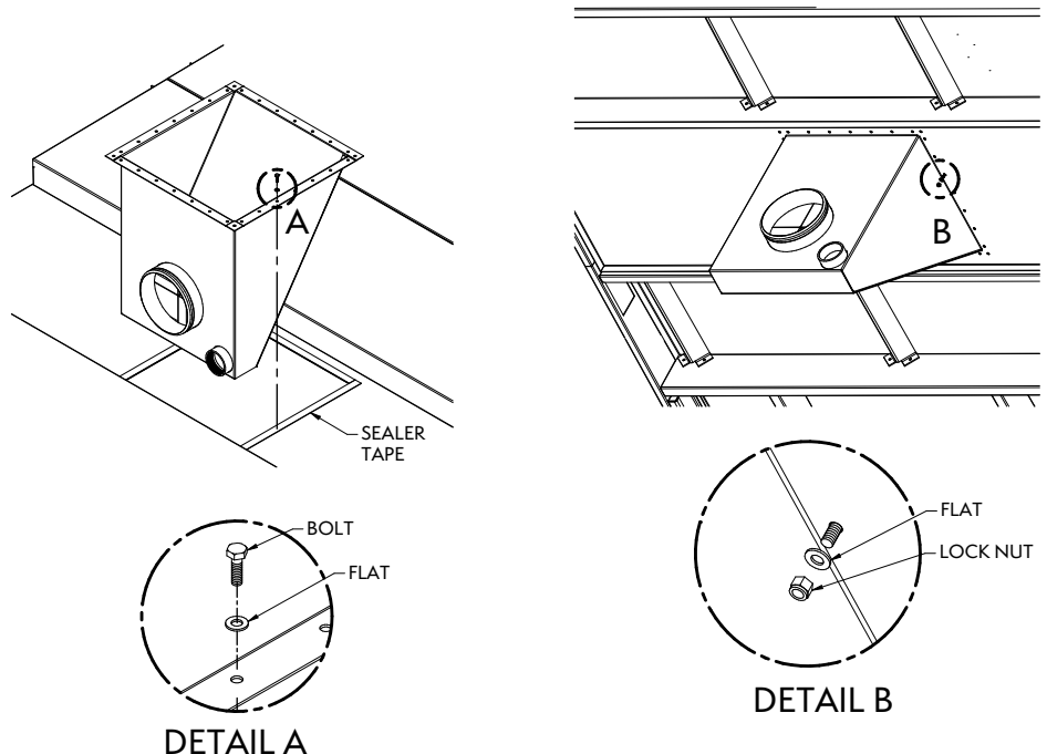
Figure 23 – Side Outlet Depressed Sump Box Installation
