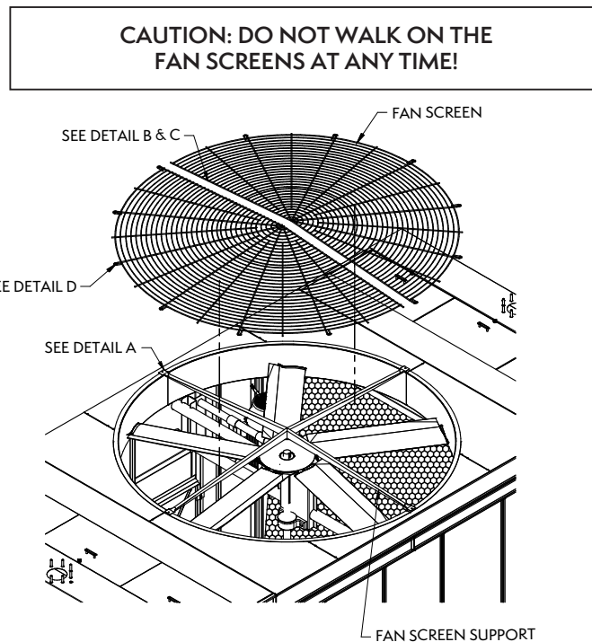
Figure 12 – Fan Screen and Fan Screen Support Frame
