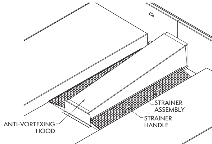
Figure 41 – Strainer Location
