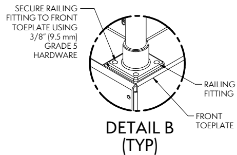
Figure 30 – Railing Securing Detail
