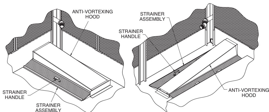
Figure 34 - Strainer Location
