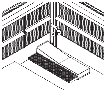
Figur 9 - ATC/W-enkel silmontering
