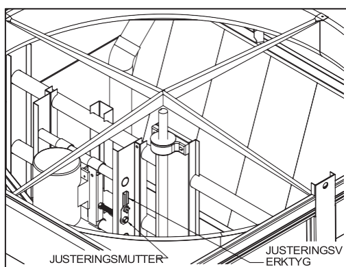
Figur 5 - Internt monterad motor, PHC-DE-enhet
