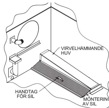
Figur 10 - LSWE/LSC-E/PMRC silmontering
